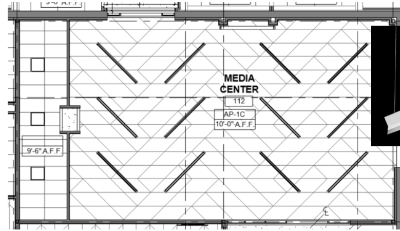
CEILING PLAN + LIGHT FIXTURE
